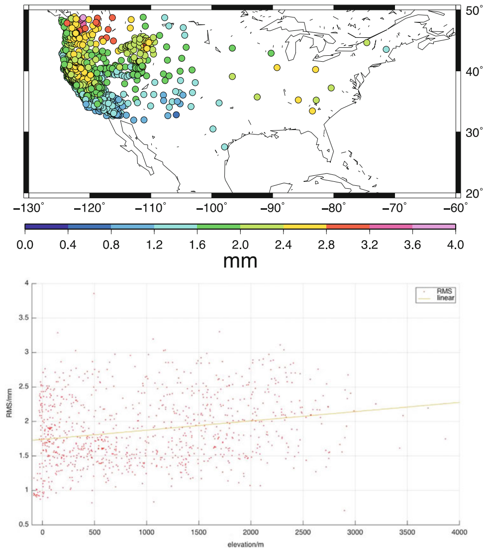
Fig. 1 (Top) RMS of the predicted weekly vertical displacement driven by NLDAS-2 Noah CWS. (Bottom) Vertical RMS of each station with respect to the elevation
